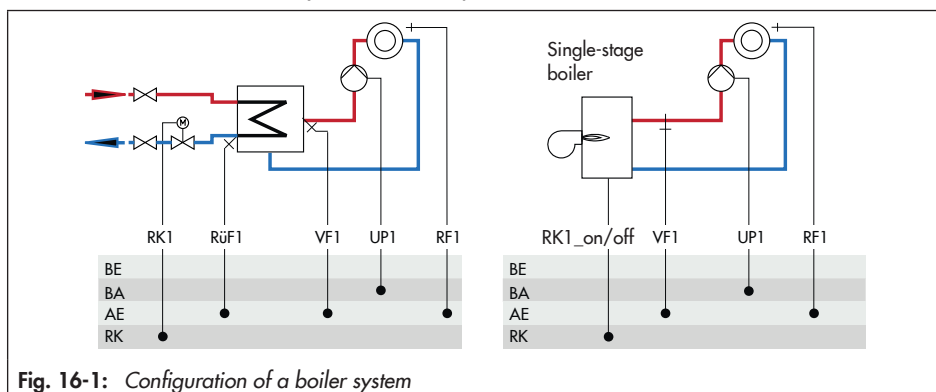
Fig. 16-1: Configuration of a boiler system
