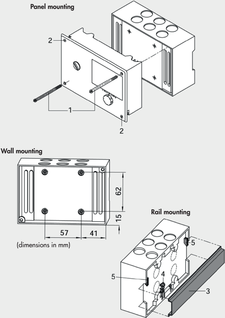
Fig. 5-1: Installation
